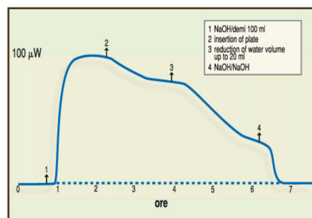
Power-time diagram of flow-mix calorimetry. Point 2: insertion of WHITE plate (7).
